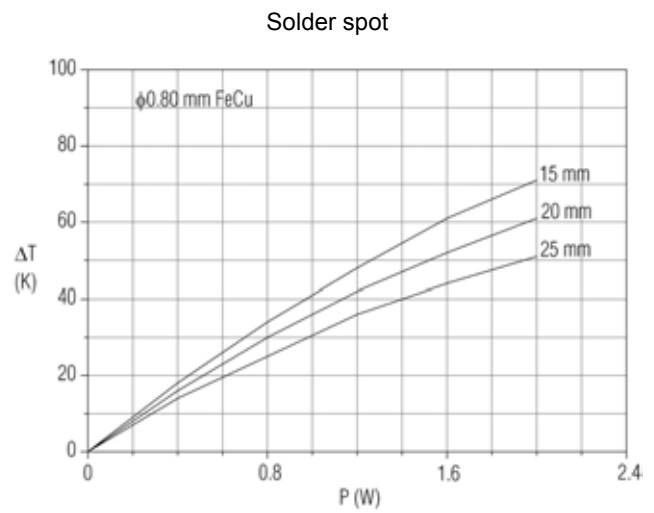
Fig. 12 - Temperature rise ( \Delta T ) at the lead end (soldering point) as a function of dissipated power at various leads. Minimum distance from resistor body to PCB = 1mm
