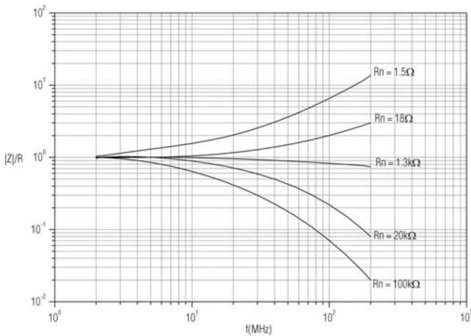
Fig. 29 - Impedance as a function of applied frequency
