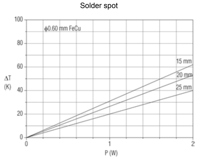
Fig. 10 - Temperature rise ( \Delta T ) at the lead end (soldering point) as a function of dissipated power at various leads. Minimum distance from resistor body to PCB = 1mm
