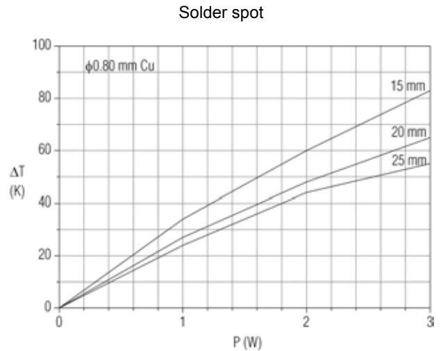
Fig. 14 - Temperature rise ( \Delta T ) at the lead end (soldering point) as a function of dissipated power at various leads. Minimum distance from resistor body to PCB = 1mm
